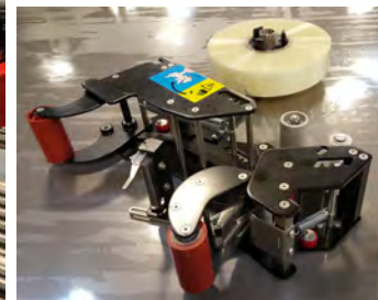
Tape Head Assembly
